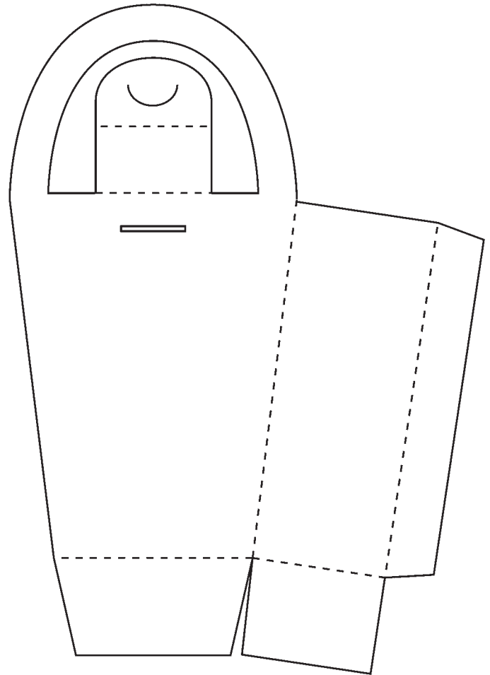
10189X Tall Bag Template (shown at 75% of actual size)
